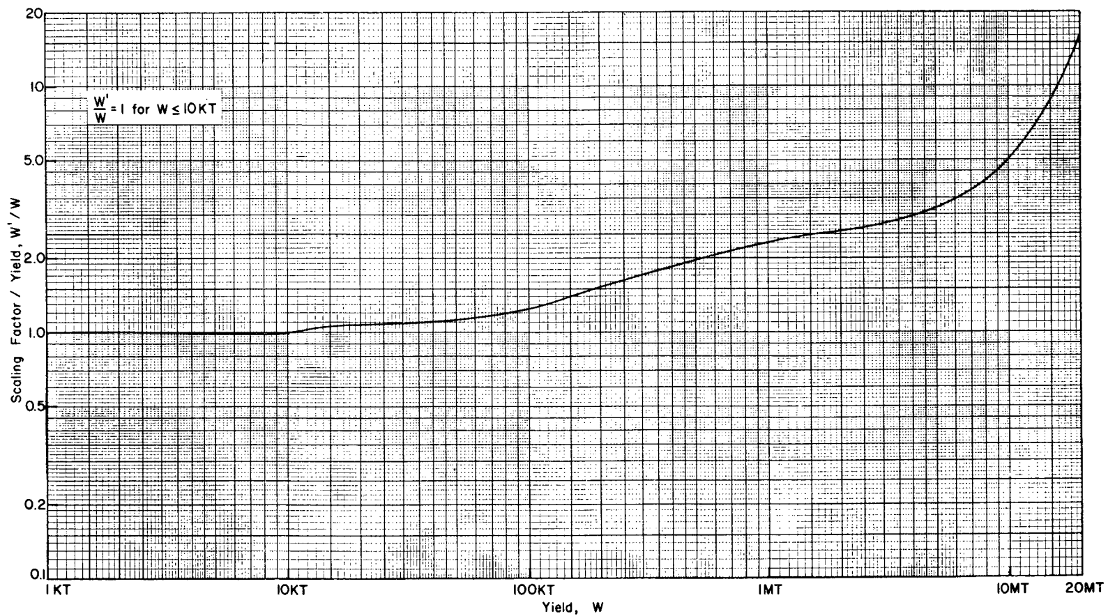
Fig. 2.15—Scaling factor for initial gamma radiation divided by yield as a function of yield (see Eq. 2.115).
